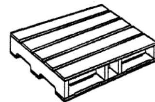
Partial 4-way entry, flush, stringer
