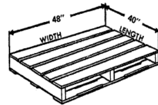
2-way entry, flush, stringer (MH1/9-04SF4048)
