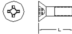
MS51959 Revision D - 316 CRES only (Flat Countersunk Head, 82 Degree, Cross-Recessed, Machine Screw)
