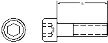
MS16995 Revision H (Hexagon Socket Head, Cap Screw)
