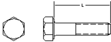
AN3 thru AN6 - Steel, CRES or Aluminum (Bolt - Machine, Aircraft, Hexagon Head)
