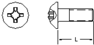
MS51957 Revision D - 316 CRES only (Pan Head, Cross-Recessed, Machine Screw)
