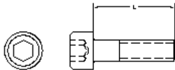
MS16995 Revision H 316 CRES only (Hexagon Socket Head, Cap Screw)
