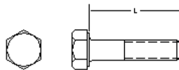
MS35307 Revision E 316 CRES only (Finished Hexagon Head, Cap Screw)
