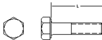
MS35307 Revision E (Finished Hexagon Head, Cap Screw)
