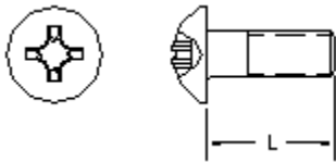
MS51957 Revision D (Pan Head, Cross-Recessed, Machine Screw)
