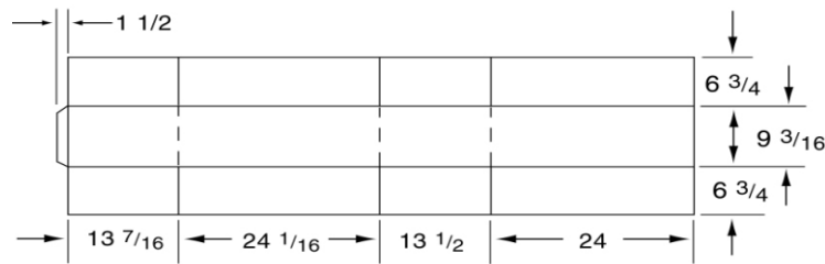
FIGURE 2 STYLE RSC FIBERBOARD (SIZE: 23 3/4 x 13 3/16 x 8 3/4 I.D.)
